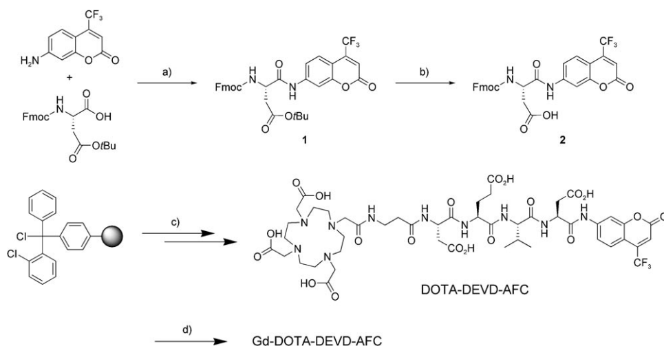
Scheme 2. Synthetic route to Gd-DOTA-DEVD-AFC. a) \text{POCl}_3 , pyridine. b) trifluoroacetic acid. c) Fmoc peptide synthesis: 2 , Fmoc-Val-OH, Fmoc-Glu(OtBu)-OH, Fmoc-Asp(OtBu)-OH, Fmoc- \beta -Ala-OH, tris- t Bu-DOTA, deprotection. d) \text{GdCl}_3 \cdot 6\text{H}_2\text{O} , 100 mM HEPES buffer (pH 7.4). Fmoc = fluorenylmethyloxycarbonyl.
